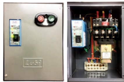
AUTOMATIC STARTER
